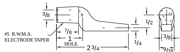
16-3821 CMW® 3 CASTING
