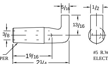
16-382120 CMW® 3 CASTING
