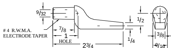
16-3820 CMW® 3 CASTING
