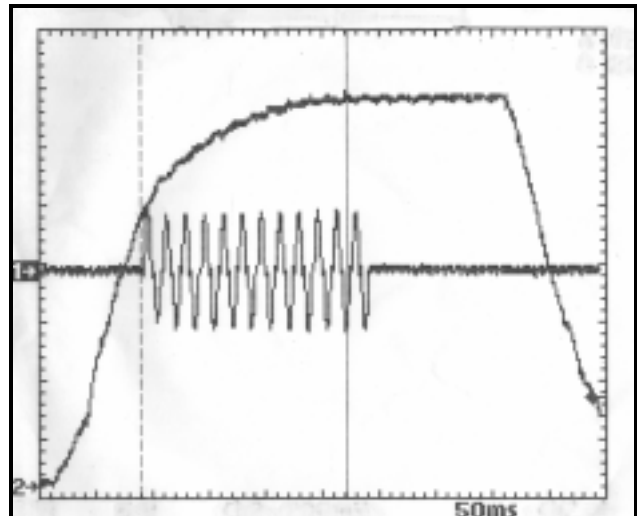
FIGURE 4: WELD BEGINS BEFORE PROPER ELECTRODE FORCE IS REACHED
